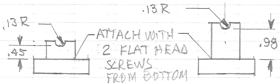
VIEW B-B
